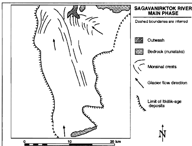
Figure 4. Drift of Sagavanirktok River main phase in upper Kuparuk River map area. Hachured lines show extent of subsequent overlap by glaciers during Itkillik time.
