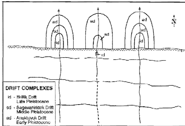
Figure 2. Drift distributions mapped along the north flank of the Brooks Range (Hamilton, 1978, 1979a, 1980), showing how extent of successive drift sheets reflect Quaternary drainage evolution in the north-central Brooks Range. Two master valleys have progressively captured drainage from the intervening valley system by headward erosion of tributaries along east-west-striking belts of erodible rock. The three valleys supported glaciers of comparable size during early Pleistocene time, but by late Pleistocene the middle valley was a relatively small glacial drainage network.
