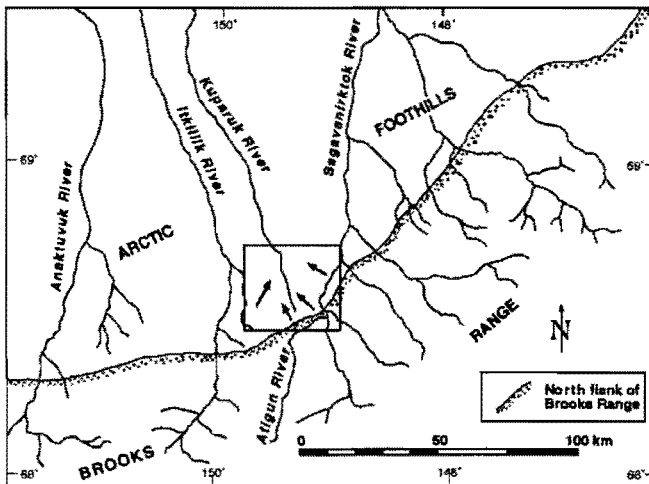
Figure 1. Itkillik-Sagavanirktok Rivers region, showing change in trend of the northern flank of the Brooks Range and asymmetric development of the Sagavanirktok drainage system. Arrows show glacial flow directions into the upper Kuparuk River region (shaded rectangle).
