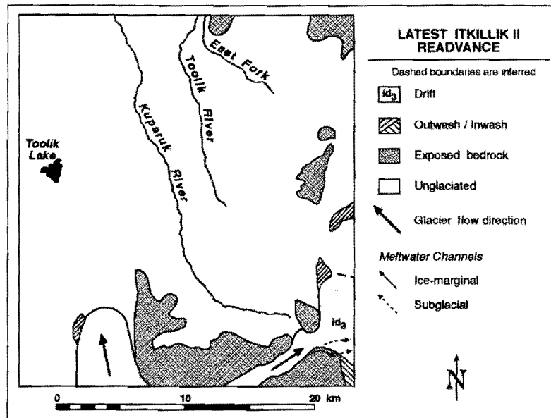
Figure 8. Drift and outwash of latest Itkillik II readvance in upper Kuparuk River map area. Unit id_3 is inwash against Atigun Valley Lobe.
