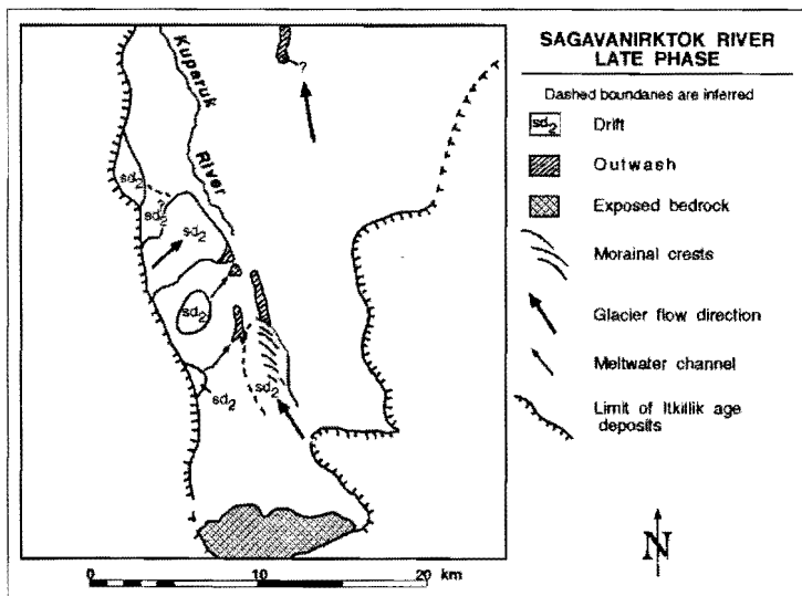
Figure 5. Drift and outwash remnants of the Sagavanirktok River late phase ( sd_2 ) in the upper Kuparuk River map area. Hachured lines show extent of subsequent overlap by glaciers during Itkillik time.
