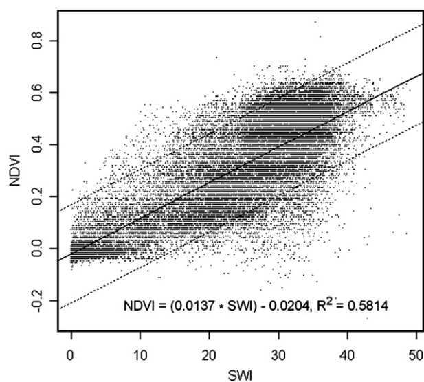
Fig. 4. Regression analysis of normalized difference vegetation index (NDVI) as a function of summer warmth index (SWI, °C), regression line (solid)±1 S.D. (dotted lines). The NDVI values are maximum NDVI from AVHRR data from 1993 and 1995. The SWI values are mean AVHRR land surface temperatures 1982–2003, buffered from coasts and excluding lakes and ice.
